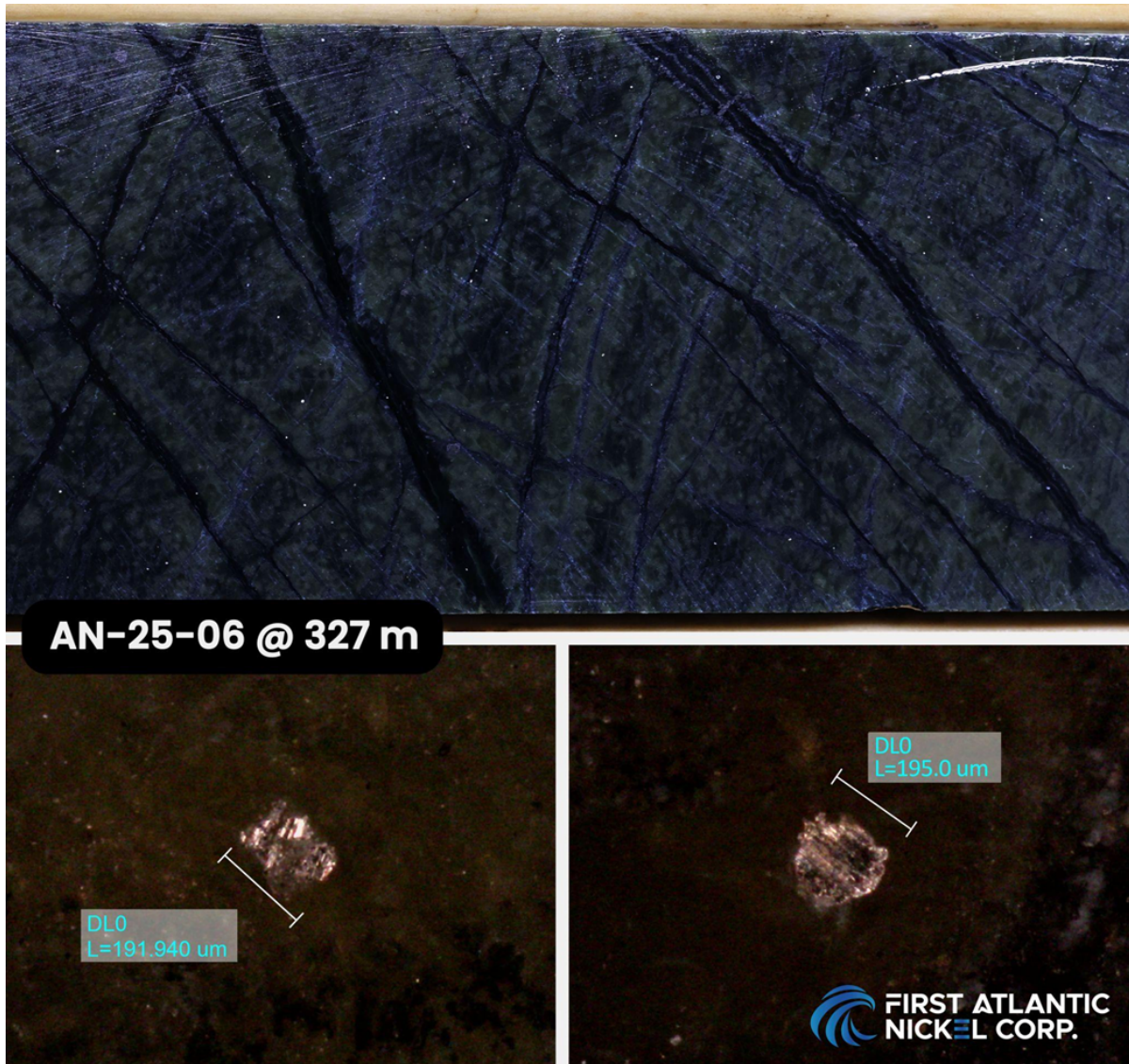
Figure 5: Drill core and microscopic images – Hole AN-25-06, 327 meters depth (RPM Zone). Top image: Drill core showing visibly disseminated awaruite (sulfur-free nickel-iron alloy) hosted in serpentized peridotite with associated magnetite veining. Bottom images: Microscopic images of awaruite grains from the same interval, with individual grains measuring up to 195 microns in size.
