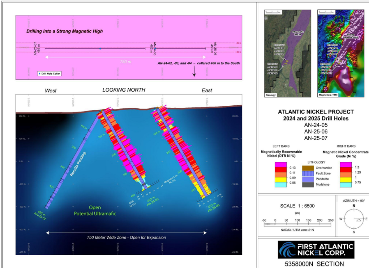
Figure 1: Section S2 - Cross sectional view of the RPM Zone, showing drill hole AN-25-06, located approximately 200 meters east of drill hole AN-24-05 on Section S2. The figure illustrates the distribution of magnetic concentrate and DTR nickel values. Drill hole AN-25-06 returned an average 1.27% nickel and 1.69% chromium in continuous metallurgical DTR magnetic concentrate over a 447.35-meter interval, with an average 9.02% mass pull and 0.11% DTR nickel.
