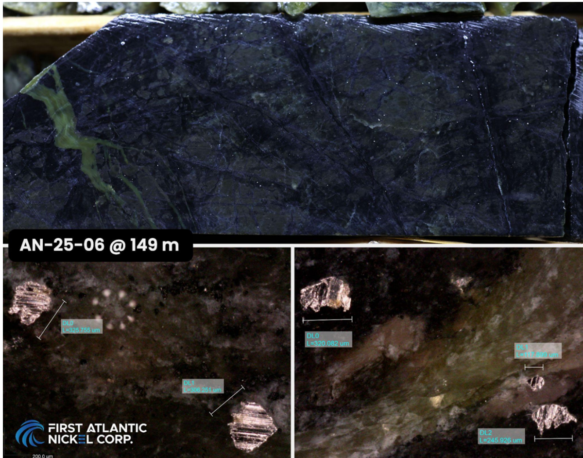
Figure 3: Drillcore and microscopic images - Hole AN-25-06, 149 meters depth (RPM Zone). Top image: Drill core showing visibly disseminated awaruite (sulfur-free nickel-iron alloy) hosted in serpentinized peridotite, with associated magnetite and serpentine veining. Bottom images: Microscopic images of awaruite grains from the same interval, with individual grains measuring up to 325 microns in size.
