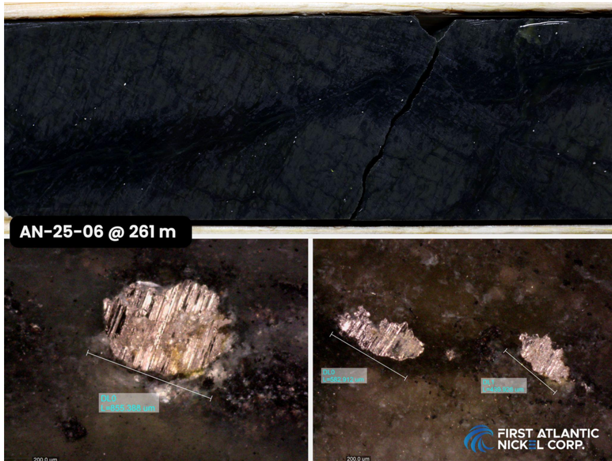
Figure 4: Drill core and microscopic images – Hole AN-25-06, 261 meters depth (RPM Zone). Top image: Drill core showing visibly disseminated awaruite (sulfur-free nickel-iron alloy) hosted in serpentinized peridotite. Bottom images: Microscopic images of awaruite grains from the same interval, with individual grains measuring up to 855 microns in size.
