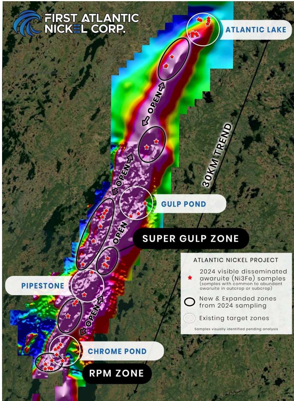
Figure 4: Atlantic Nickel target zones including RPM and Super Gulp showing 2024 sampling with visible awaruite (nickel-alloy) locations over the 30 km nickel ultramafic magnetic trend (background TMI magnetics).
