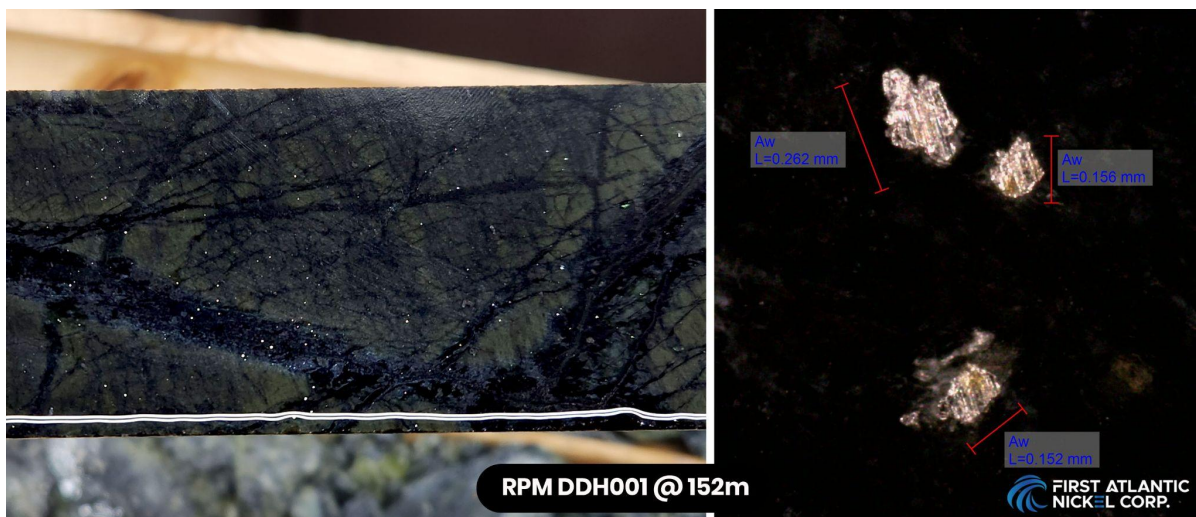
Figure 2: RPM DDH001 (24-AN-02) at 152 meters showing coarse grains of nickel-iron alloy (awaruite). Left image shows drill-core with disseminated awaruite in serpentized ultramafic cut by serpentine-magnetite fracture fillings and veinlets; Right image shows microscope photo of nickel alloy grains ranging from 152 - 262 microns.
