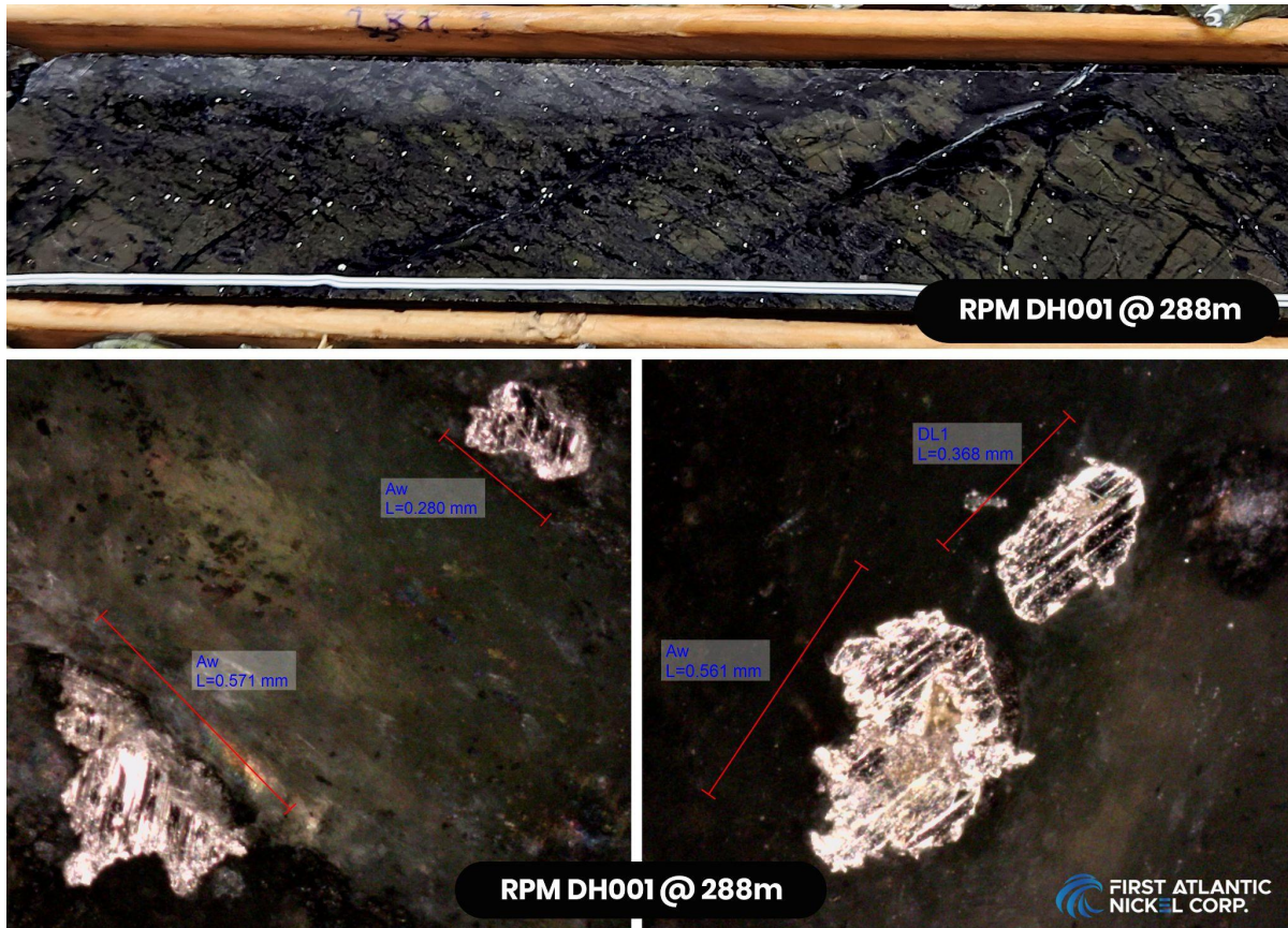
Figure 3: Top image showing coarse grained visible nickel-iron alloy (awaruite) in serpentinized ultramafics within the first drillhole at RPM Zone DDH001 (24-AN-02) at 288 meters downhole; bottom images are microscope photos showing large grains of nickel-iron alloy ranging from 280 microns to 571 microns at 288 meters
